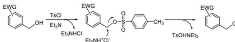
Figure 2. S_N2 reaction formation of EWG-containing benzyl chlorides (TsCl is arbitrary, MSC works too) 3,20,21 .
